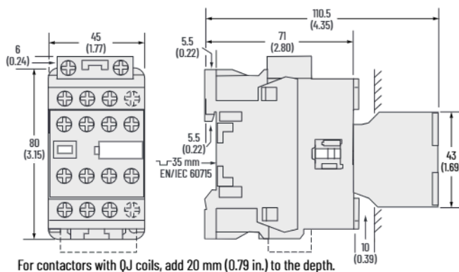
Figure 39 - 100(S)-E09...100(S)-E16 Contactors with Low-consumption Coils and Front-mounted Auxiliary Contact
