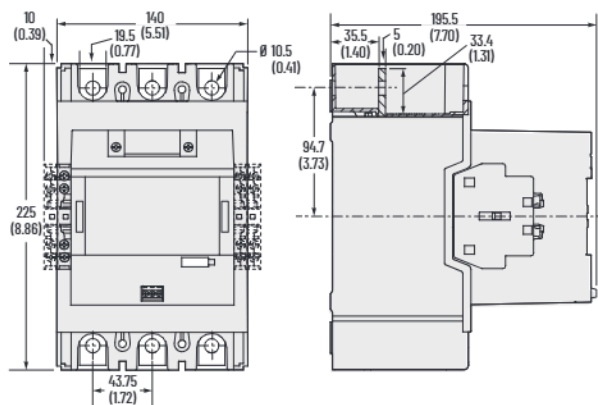
Figure 85 - 100(S)-E265E...100(S)-E370E Contactors with PLC Input
