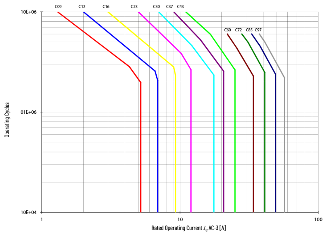
Figure 15 - AC-3, Switching of Squirrel-cage Motors while Starting; U_e = 690V
