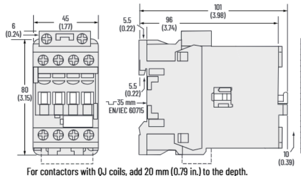
Figure 46 - 100-E26...100-E38 4-Pole Contactors with Low-consumption Coils
