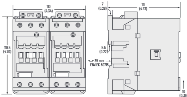
Figure 60 - 104-E40...104-E65 Reversing 3-Pole Contactors
