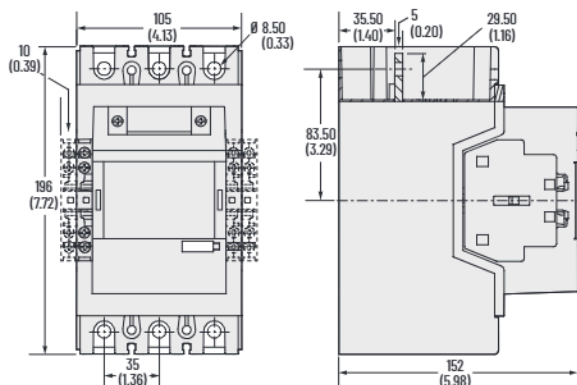
Figure 81 - 100(S)-E190E, 100(S)-E205E Contactors with PLC Input
