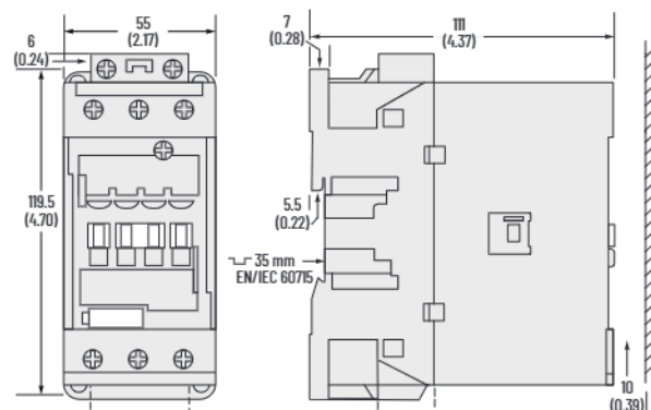
Figure 58 - 100(S)-E40...100(S)-E65 3-Pole Contactors with Front-mounted Auxiliary Contact
