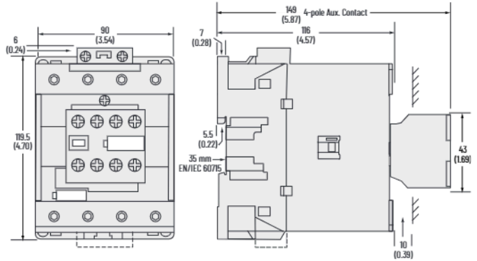
Figure 73 - 100-E80 4-Pole Contactors with Side-mounted Auxiliary Contact
