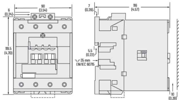
Figure 71 - 100-E80 4-Pole Contactors
