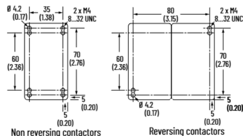
Figure 42 - Drilling Template for 9...16 A Contactors
