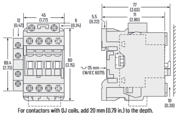
Figure 39 - 100(S)-E09...100(S)-E16 Contactors with Low-consumption Coils and Front-mounted Auxiliary Contact
