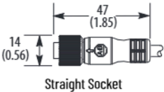
Straight Socket
