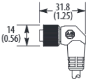
Right-angle Socket
