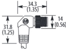
Right-angle Plug
