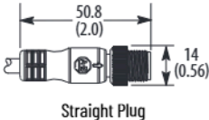
Straight Plug
